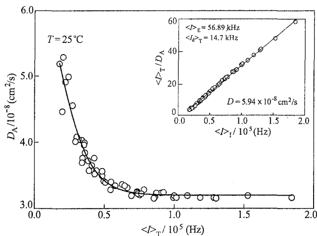
Fig. 2 Time-average scattered intensity \langle I \rangle_T dependence of apparent diffusion coefficient D_A of hybrid PNIPAM gel at 25°C, where D_A was obtained from the initial slope of the intensity-intensity time correlation function. The inset shows a decomposition plot on the basis of Eq. (3).
