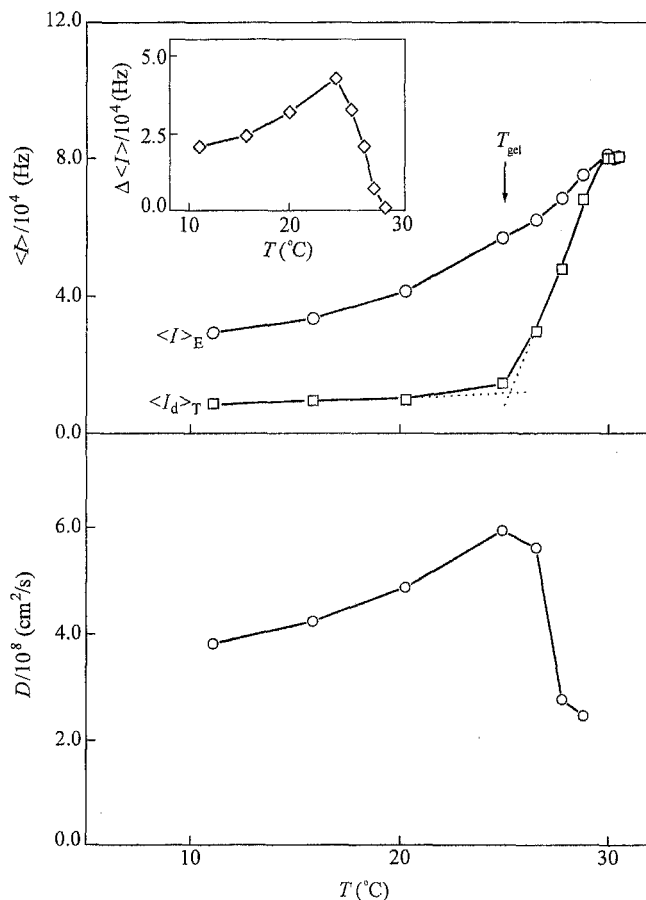
Fig. 3 Temperature dependence of ensemble-average scattered intensity \langle I \rangle_E , time average dynamic component of scattered intensity \langle I \rangle_T and collective diffusion coefficient D of hybrid PNIPAM gel. The arrow shows the gelation temperature T_{\text{gel}} observed by a flow test. The inset is the temperature dependence of the intensity difference ( \Delta I ) between \langle I \rangle_E and \langle I \rangle_T .
